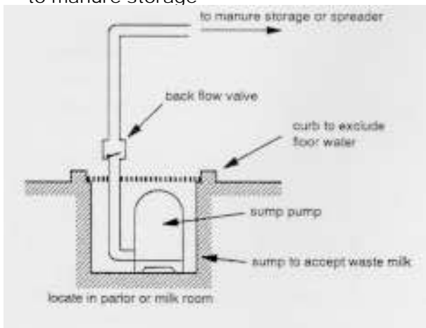
Figure 3. Sump for pumping waste milk to manure storage
