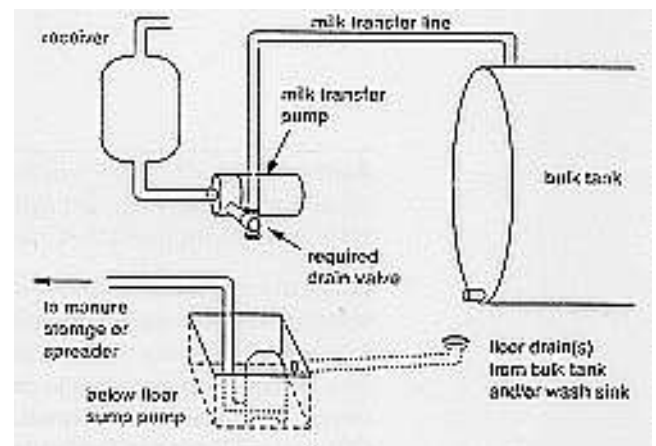
Figure 2. Collection sump for pumping waste milk to manure storage
