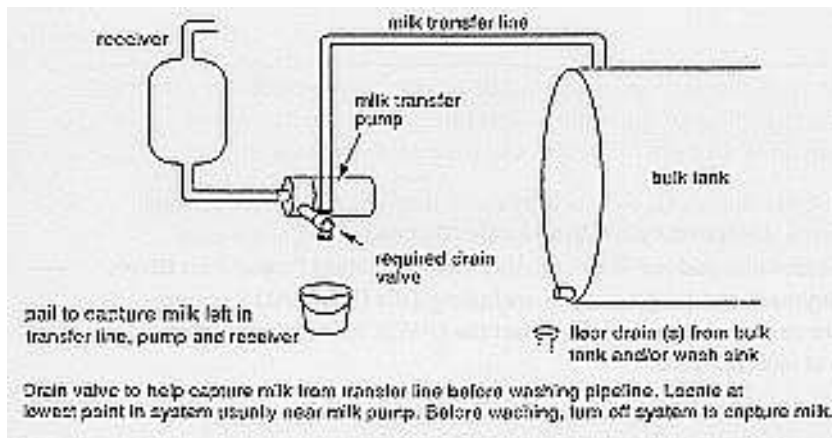
Figure 1. Residual milk from a transfer line captured in a bucket
